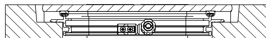
SECTION B-B
